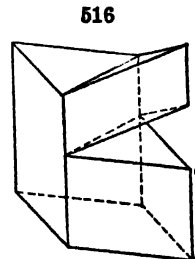
Artificial Twinning in Calcite
